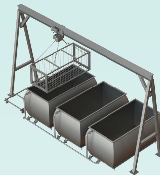
Molds Washing Unit
