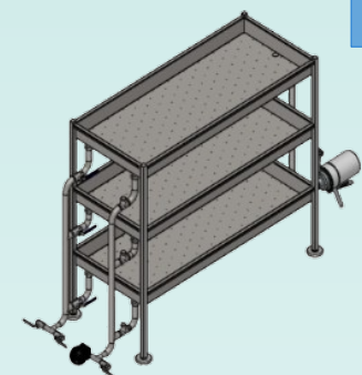
Kaymak Cooking Trolley (Steam)
